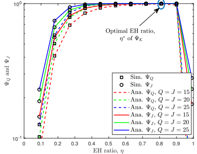
Fig. 6: Impact of the EH ratio \eta on OSCP of the BIH and BIL, with \gamma_U = 4 (dB), h_U = 30 (m), \Omega = 3 , and \psi = 0.4 .
