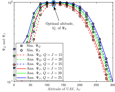
Fig. 5: Impact of the UAV's altitude h_U on OSCP of the BIH and BIL, with \gamma_U = 4 (dB), \eta = 0.1 , \Omega = 3 , and \psi = 0.4 .
