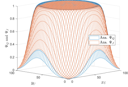
Fig. 7: Impact of the UAV's position (x_U, y_U) on OSCP of the BIH and BIL, with Q = J = 20 , \gamma_U = 2 (dB), h_U = 20 (m), \eta = 0.05 , \Omega = 3 , and \psi = 0.4 .
